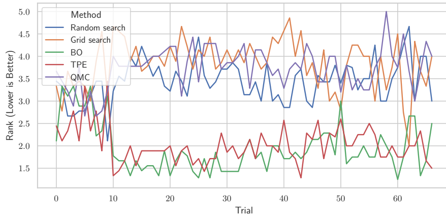
Figure 1. Ranks-over-time of the benchmarked HPO methods over the progress of the optimization, aggregated over 10 independent runs for each of 9 datasets.
