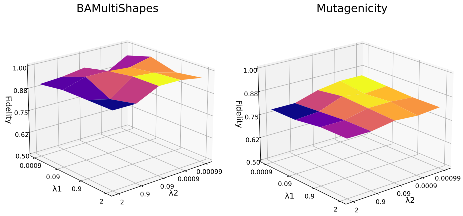
Fig. 2. How does the selection of \lambda_1 and \lambda_2 impact Fidelity?
