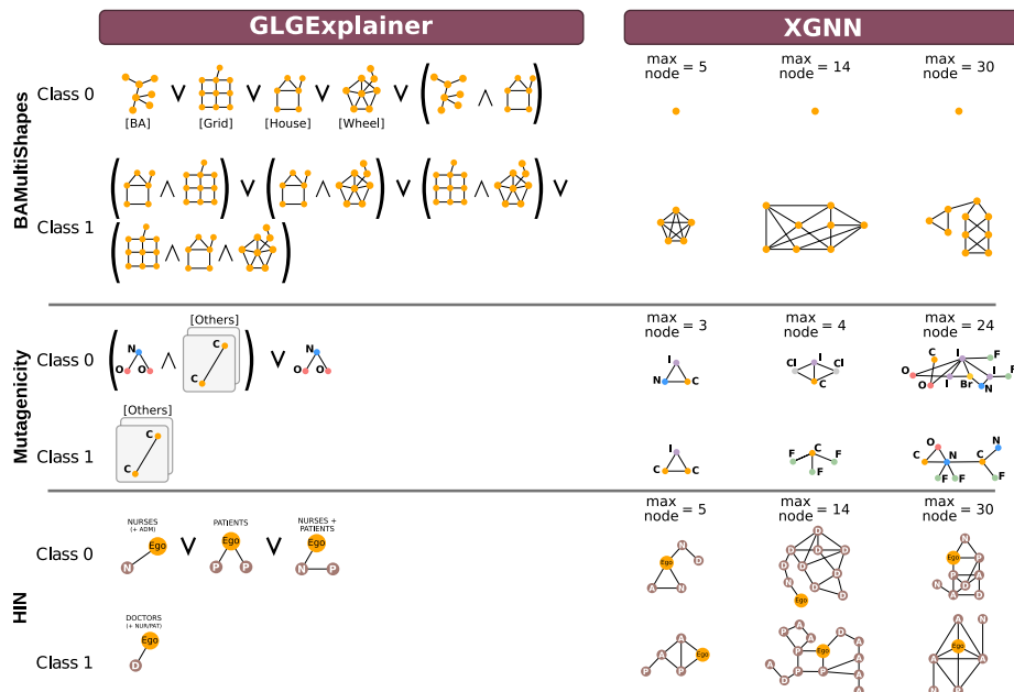
Fig. 3. Global explanations of GLGExplainer (ours) and XGNN. For Class 0 of BA-MultiShapes, XGNN was not able to generate a graph with confidence \geq 0.5 . Note that for each clause, missing concepts are implicitly negated.
