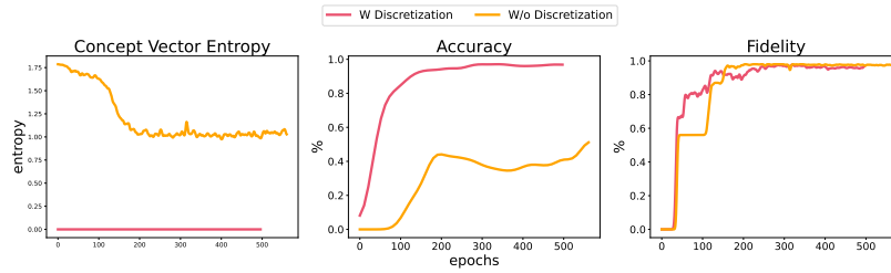
Fig. 4. Impact of the Discretization Trick. Each run is halted with early stopping on the validation set.
