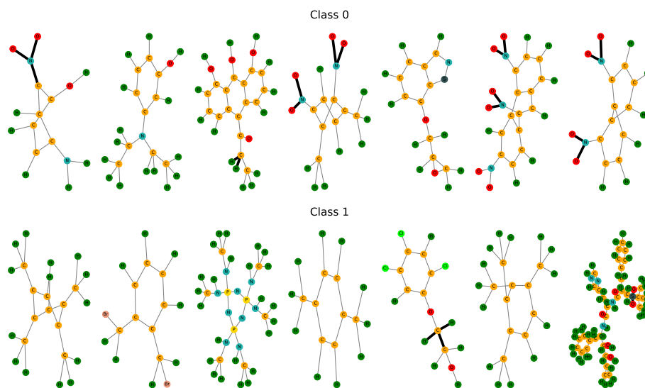
Fig. 4. Random examples of input graphs along with their explanations in bold as extracted by PGExplainer, for Mutagenicity
