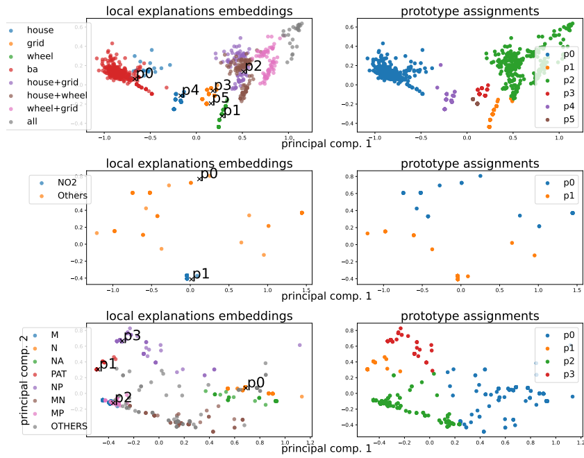
Fig. 6. 2D PCA-reduced embedding for, respectively, BAMultiShapes and Mutagenicity and HIN
