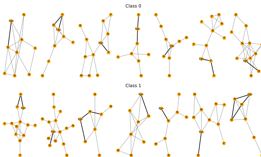
Fig. 5. Random examples of input graphs along with their explanations in bold as extracted by PGExplainer, for HIN
