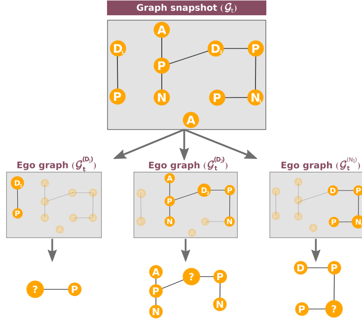
Fig. 1. Extraction of ego graphs in Hospital Interaction Network (HIN).
