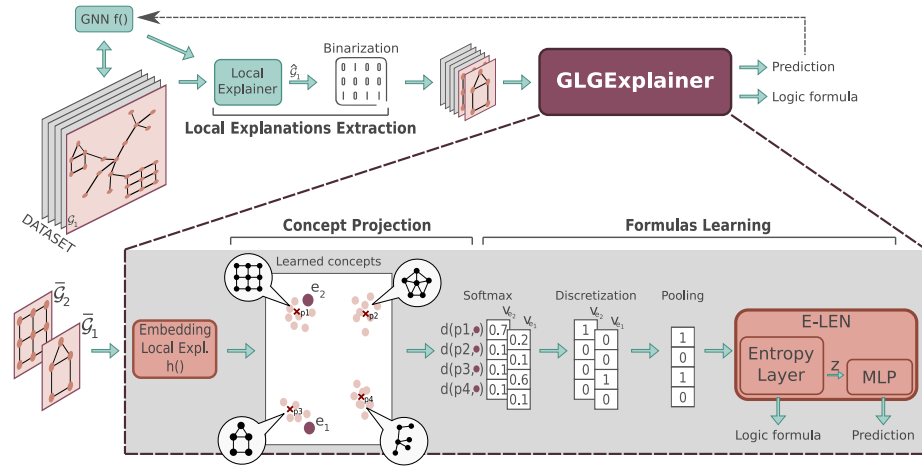
Fig. 1. Illustration of the proposed method.
