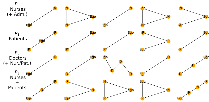
Fig. 9. Five random local explanations for each concept in HIN.
