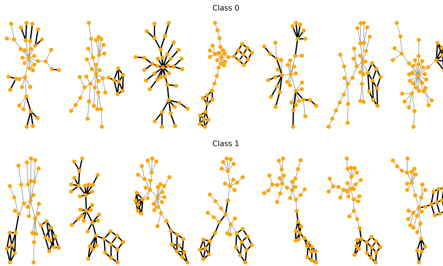
Fig. 3. Random examples of input graphs along with their explanations in bold as extracted by PGExplainer, for BAMultiShapes.
